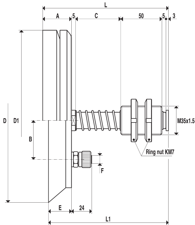
Cup holder with rapid straight fitting for plastic hose
